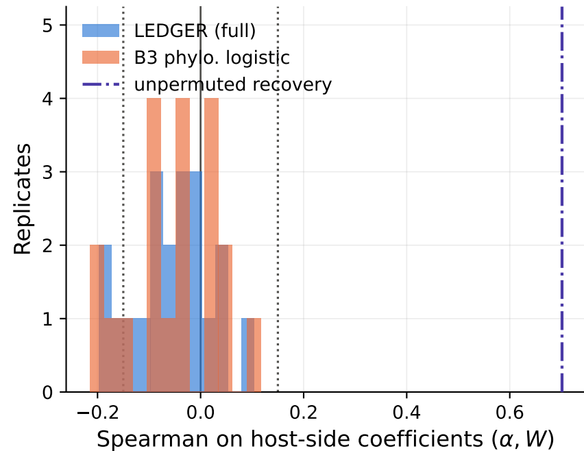
global residual \text{corr}(D) = -0.007
