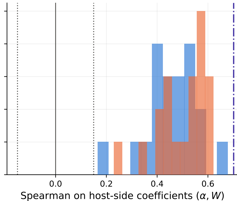
within lineage residual \text{corr}(D) = 0.489
